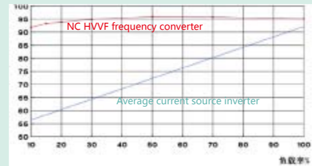
Figure 4 Power factor
