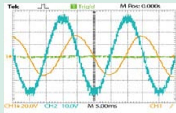
Figure 2 Waveform of output voltage and current
