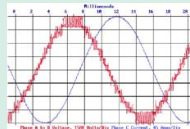
Figure 5 Multi-level, pulse width modulation of the output waveform
