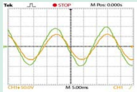
Figure 1 Waveform of input voltage and current
